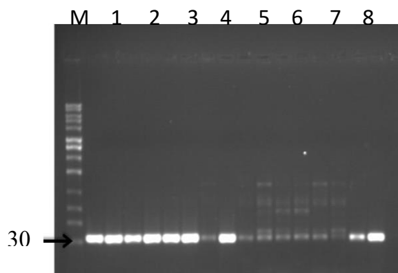
Fig 3. PTYv787/PTYc1121 primer pairs' amplicon of size 300 bp for TYLCV in 8 tomato genotypes from UCC represented by lanes 1-8 (1- K100, 2- K027, 3- K116, 4- K005, 5- K202, 6- LV, 7- K213 and 8- K042). C denotes the negative control while M is 1 kb DNA Ladder.
