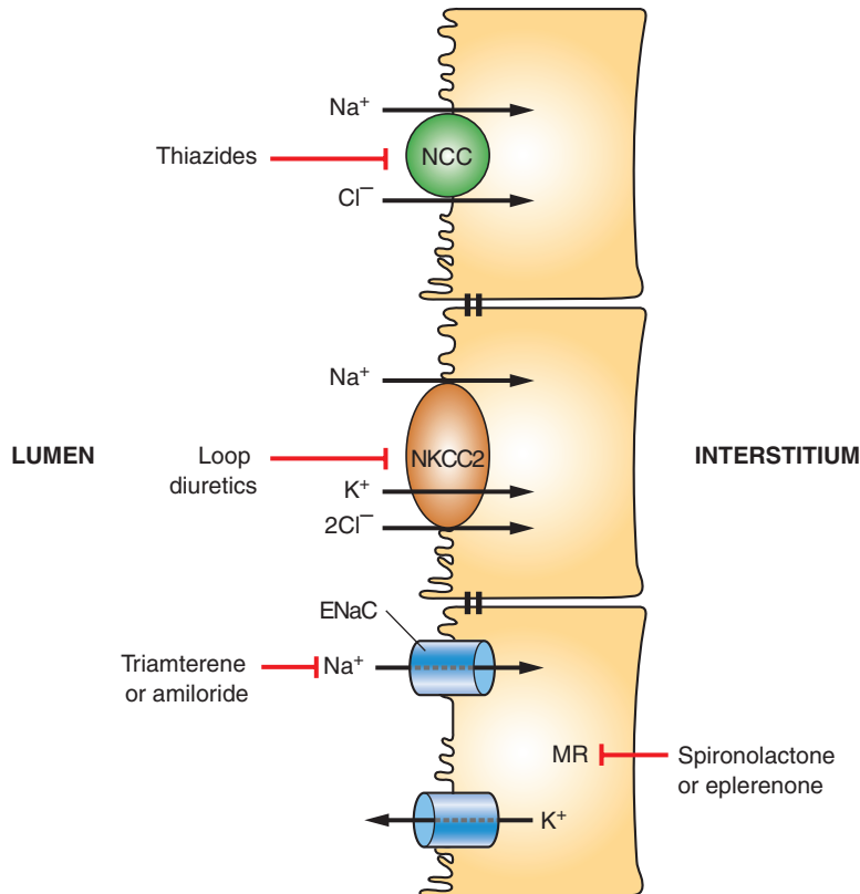
FIGURE 3.2. The molecular targets of thiazide and loop diuretics are transmembrane cotransporters, whereas the molecular target of amiloride is a specific Na + channel.
