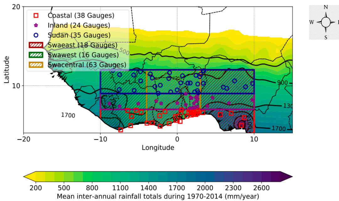
Figure 2. Long-term daily rainfall series used to quantify rainfall over six sub-divisions over the SWA; mean annual rainfall totals over the West African region (shading) from rain gauge data are also represented for the period 1970–2014.
